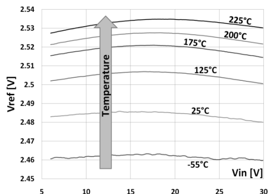
Figure 4: Typical internal voltage reference dependence on V_{in} and temperature.
