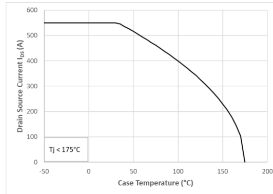
Figure 18: Continuous Drain Current Derating vs Case temperature
