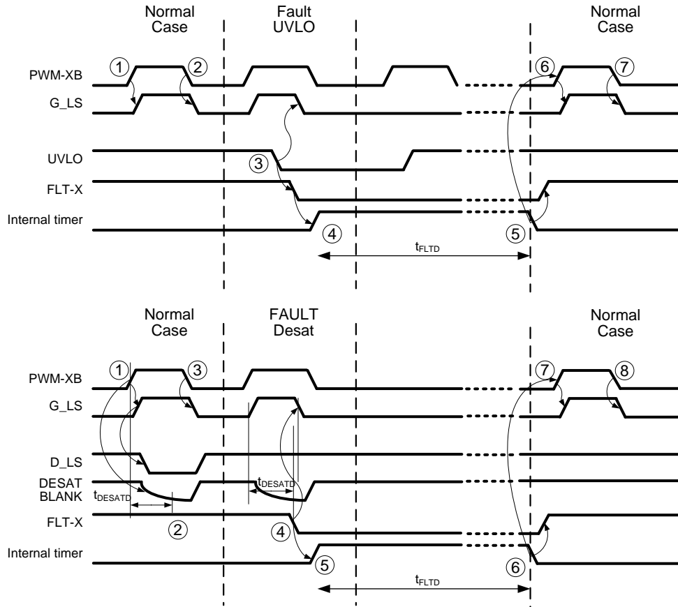
Figure 25: Timing diagram CXT-PLA3SA12550A low-side gate driver behaviour
