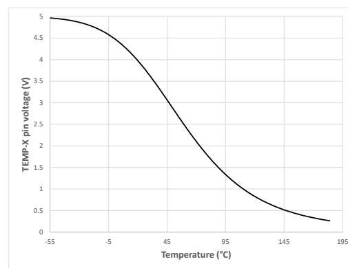
Figure 22: TEMP-X voltage vs temp
