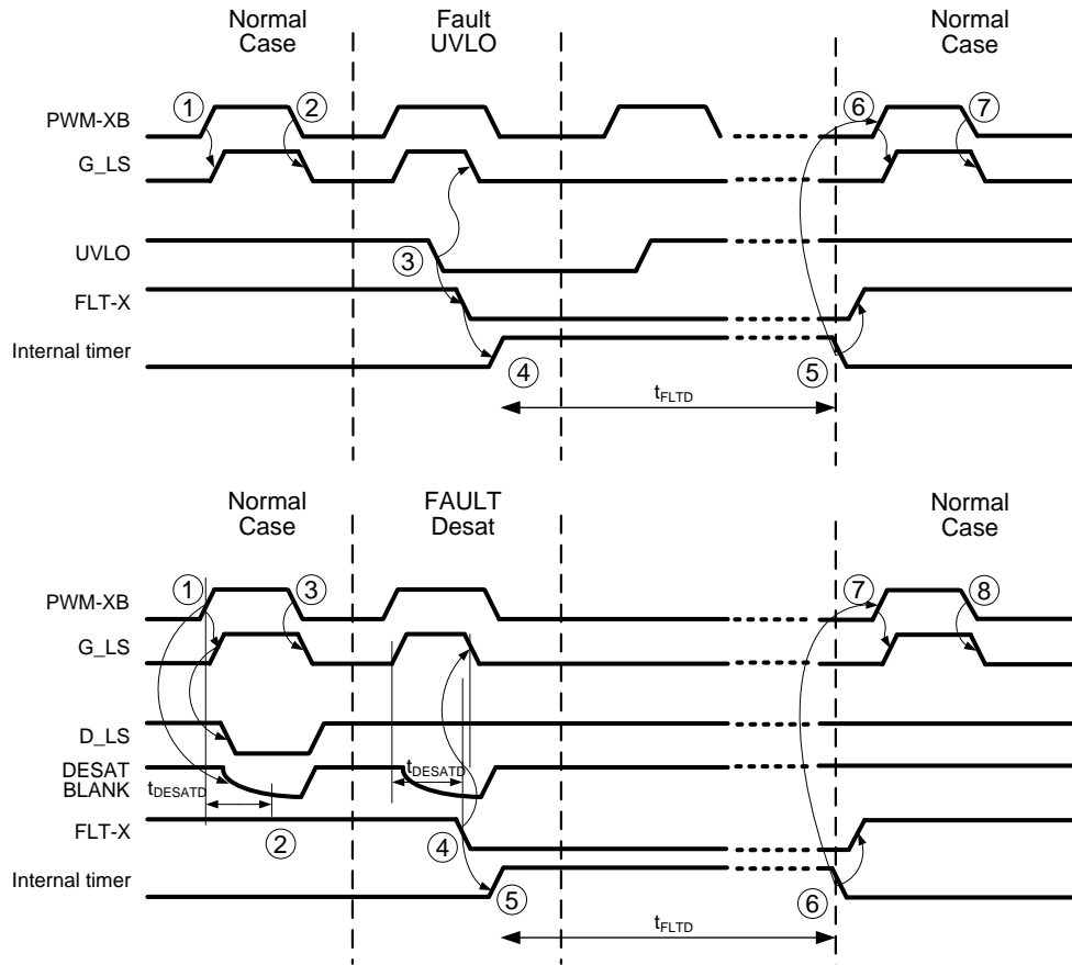
Figure 24: Timing diagram CXT-PLA3SA12450A low-side gate driver behaviour
