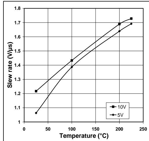
Slew Rate vs. Temperature for V_{DD} = 5/10V
