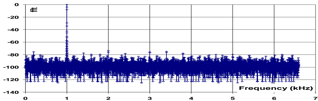
Normalized fft (dB) @ 25°C – 13.1kS/s (internal CK)
