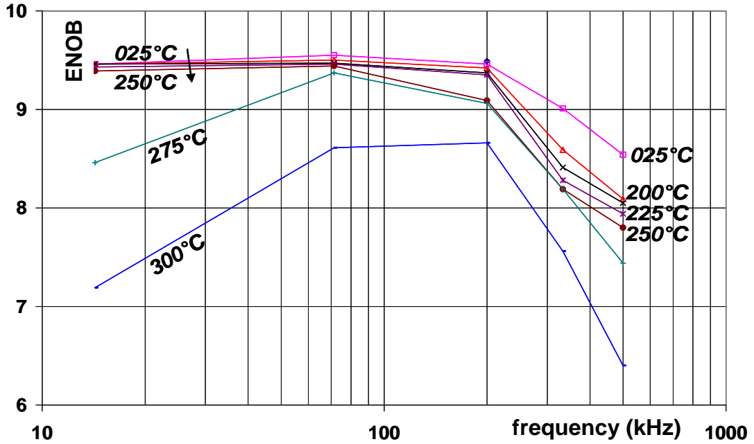
Figure 8: Typical ENOB over Temperature vs. external CK frequency
