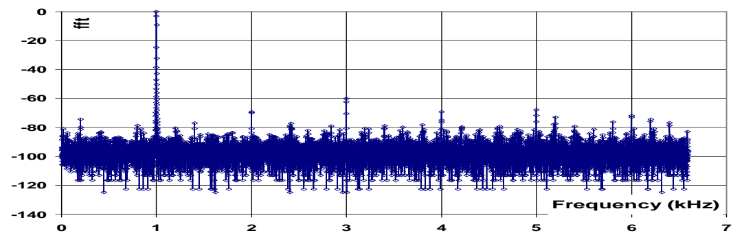
Normalized fft (dB) @ 300°C – 13.1kS/s (external CK)
